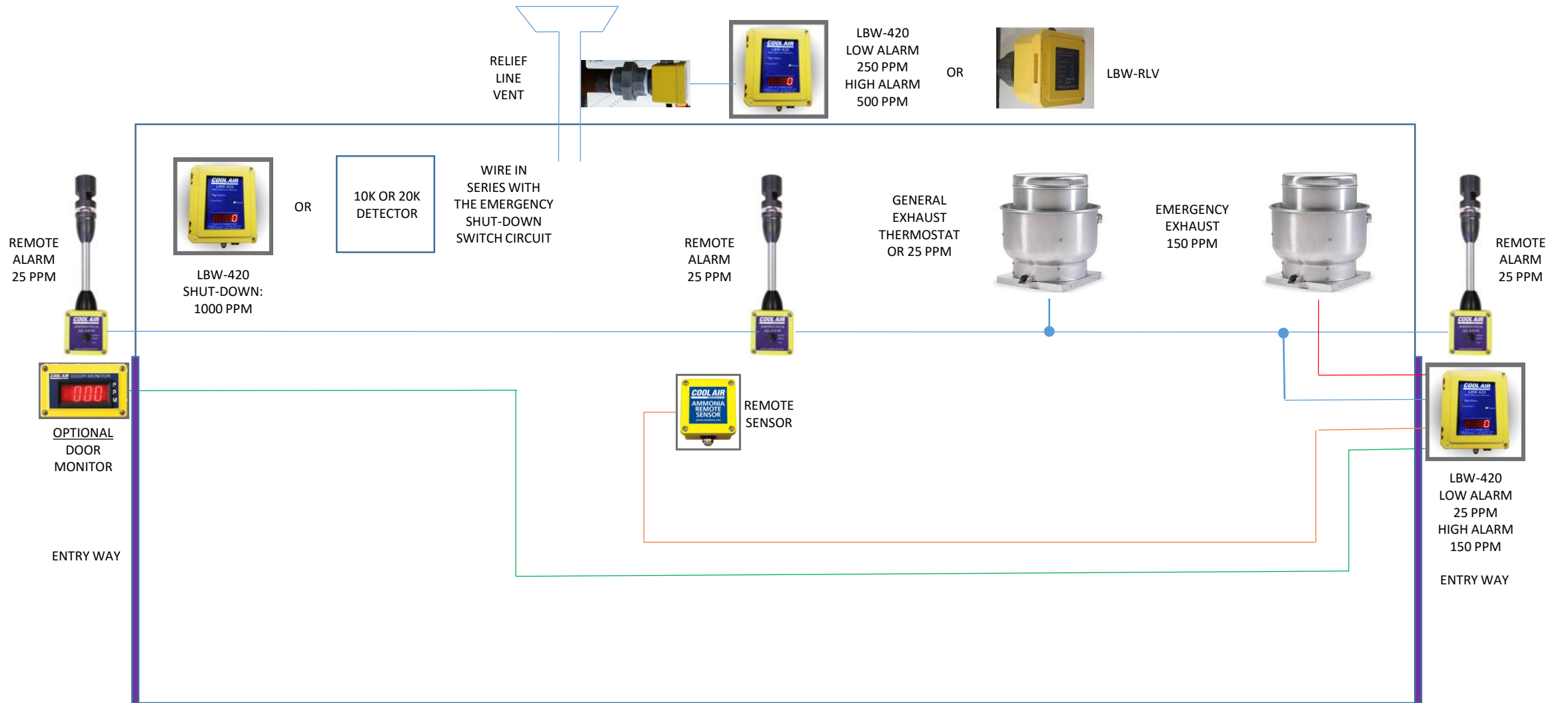
2 ND EXAMPLE: ENGINE ROOM WITH LBW-420'S, REMOTE SENSOR, DOOR MONITOR, & REMOTE ALARMS
